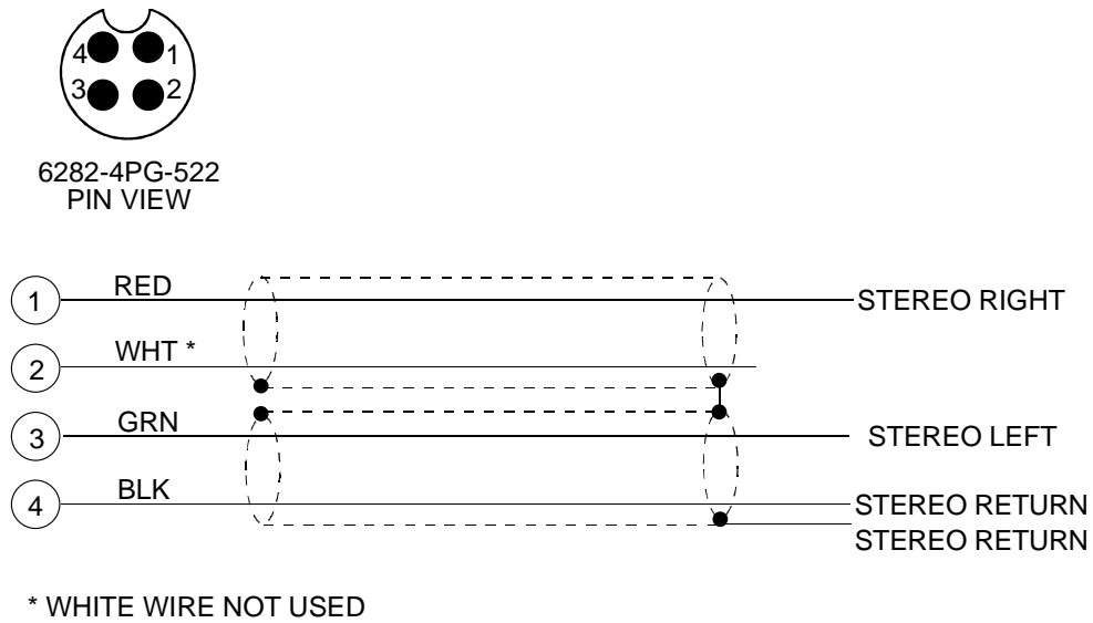
Figure 2: C98-30AX Cable Schematic
