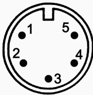
PIN VIEW NC5MX-B
