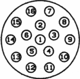
PIN VIEW S104A086-140 E3104.2/4.7+B
