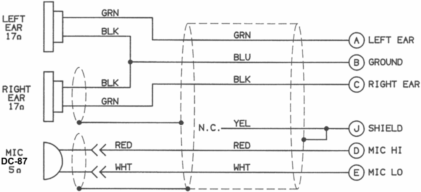
PIN VIEW AMPHENOL PT06E-12-10P (SR)
