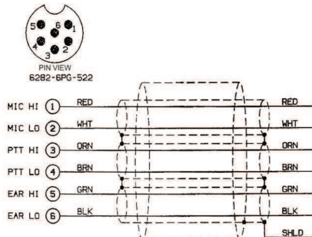
Figure 1. C98-20RD Radio Interface Cable Schematic
