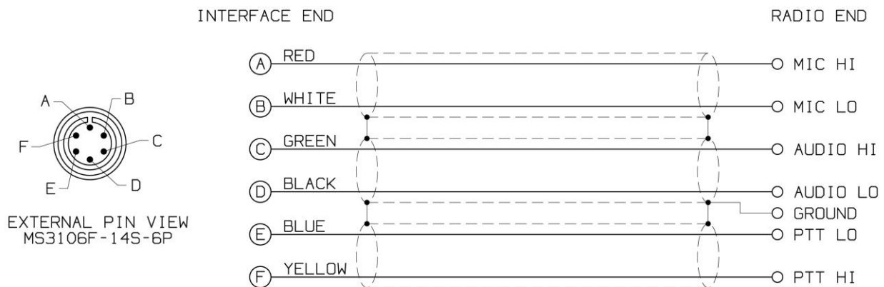
Figure 1. Model C3821 Radio Interface Cord Schematic Diagram.
