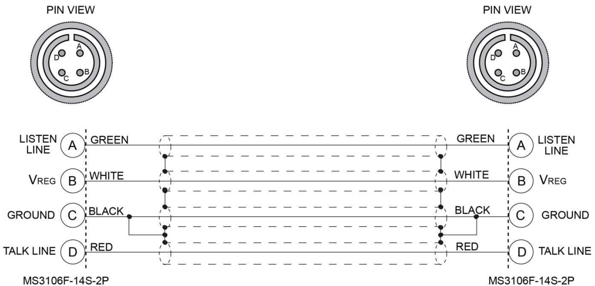
Figure 1. Model C38-XX System Jumper Cord Schematic Diagram
