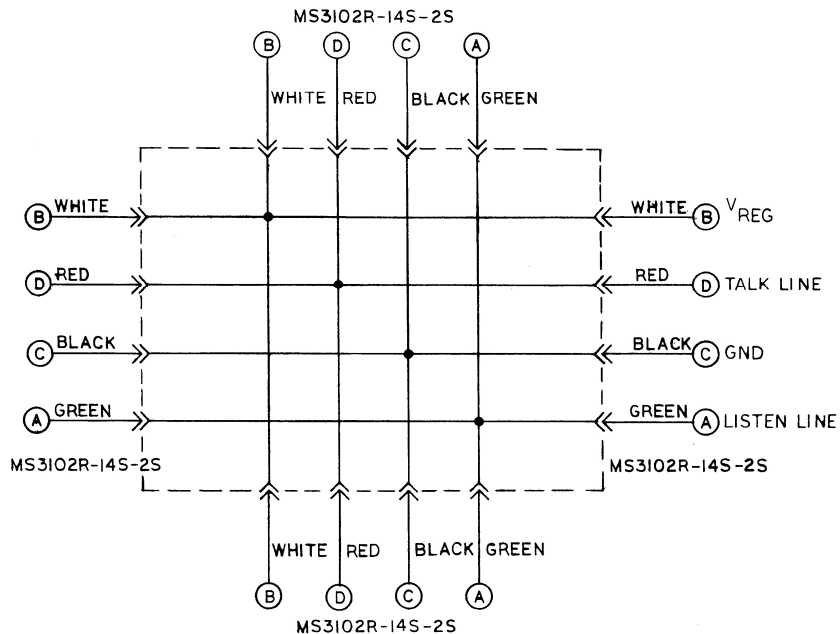
Figure 1. Model U3803 Remote Junction Module Schematic Diagram.
