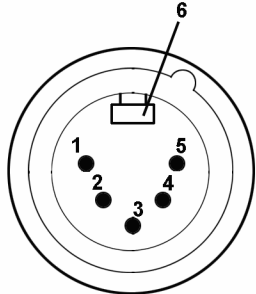
EXTERNAL PIN VIEW NC5MX-B
