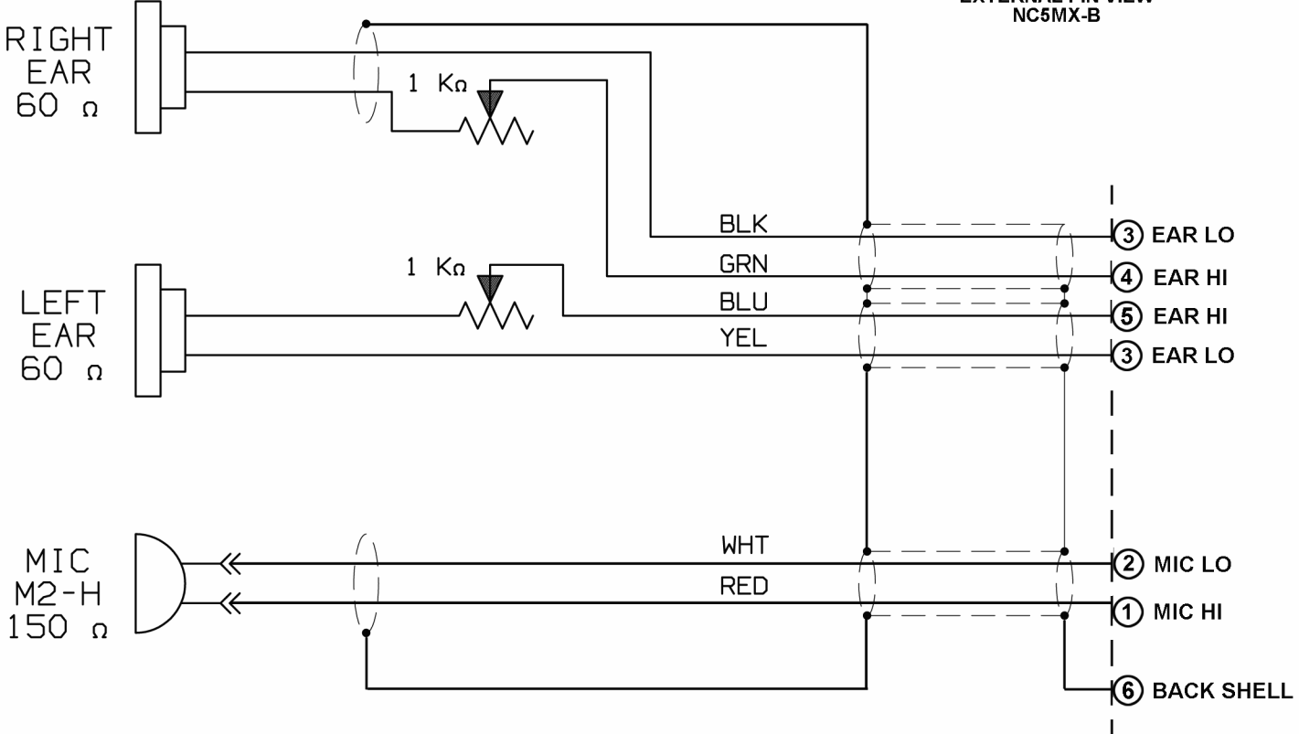
EXTERNAL PIN VIEW NC5MX-B
