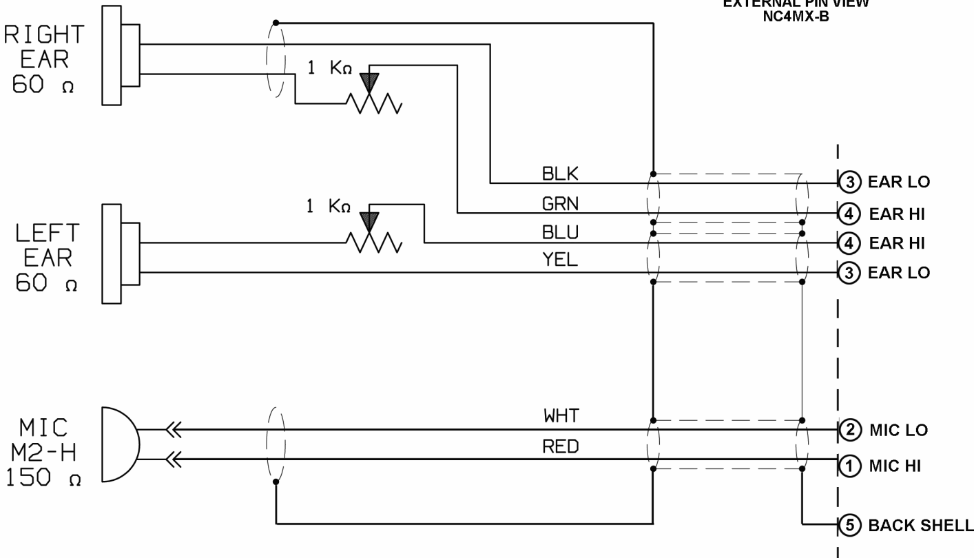
EXTERNAL PIN VIEW NC4MX-B
