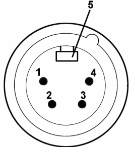
EXTERNAL PIN VIEW NC4MX-B
