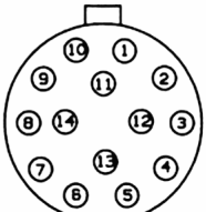
EXTERNAL PIN VIEW PHW.28.314.XLAD52Z
