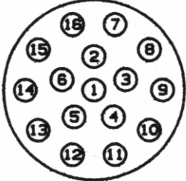
PIN VIEW S104A086-140 E3104.2/4.7+B
