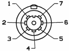
EXTERNAL PIN VIEW NEXUS AP-117PLR-CP
