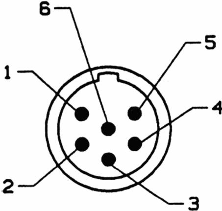
TB6M SWITCHCRAFT PIN VIEW
