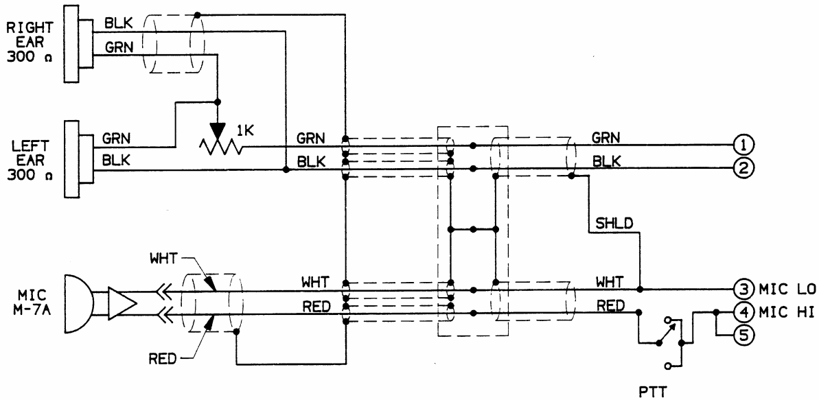
XLR-5-12C SOLDER VIEW
