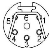
09227P-81 Solder View
